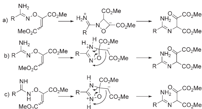
Scheme 4. a)–c) Plausible stepwise nucleophilic mechanisms.
