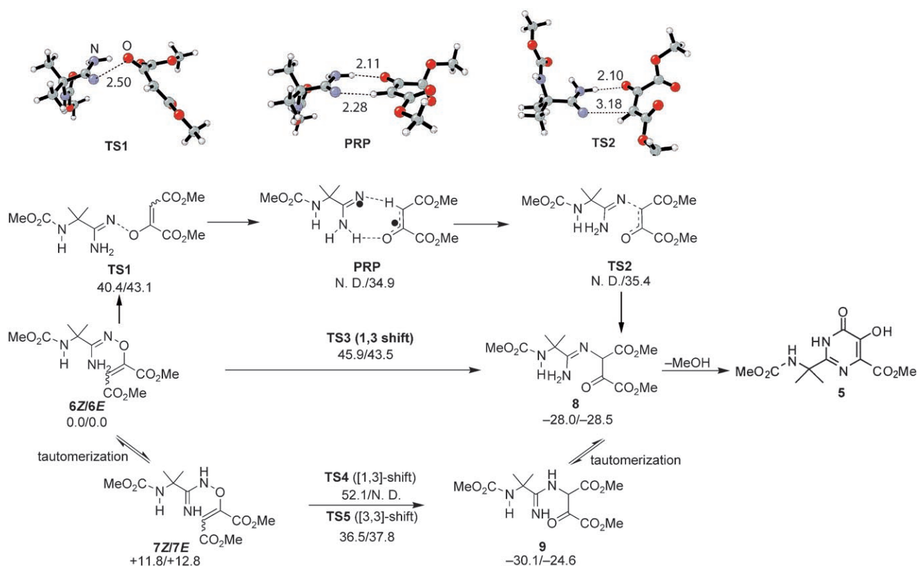
Scheme 3. Corrected B3LYP energies and relevant transition structures and intermediates in the possible rearrangement mechanisms of amidoximes 6Z and 6E . All energies [kcal mol -1 ] are referenced to 6Z and 6E . Pictures are for structures in the stepwise rearrangement of 6E . (N.D. = not determined.)
